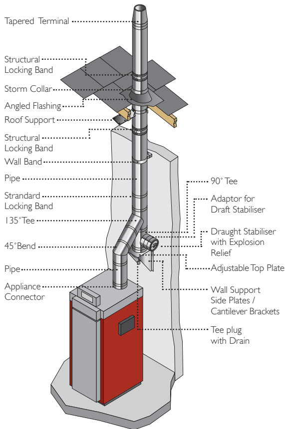
TYPICAL BIOMASS INSTALLATION FROM TOP OUTLET USING ICS SYSTEM CHIMNEY
