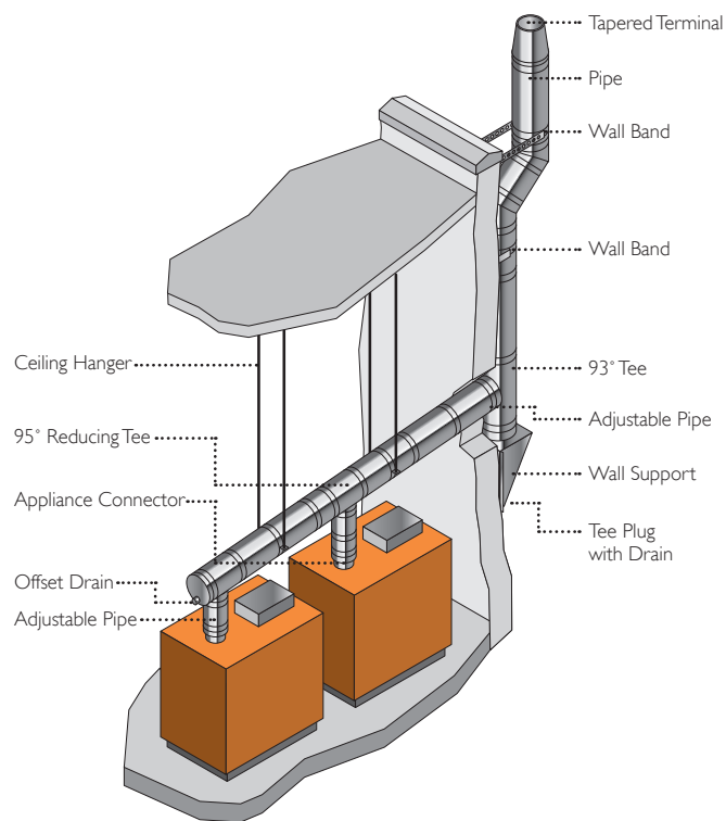
TYPICAL CONDENSING BOILER INSTALLATION USING ICS PLUS
