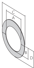
2 - Piece Trim Collar 45°
