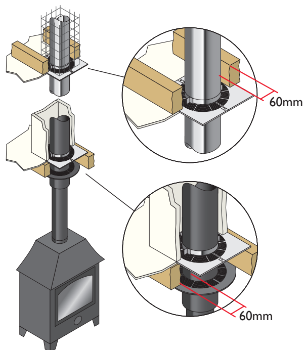
TYPICAL INSTALLATION OF ICS25 THROUGH A COMBUSTIBLE FLOOR & SHAFT
