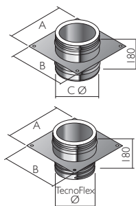
Anchor Plate - TecnoFlex Plus Screw Fit Connection
