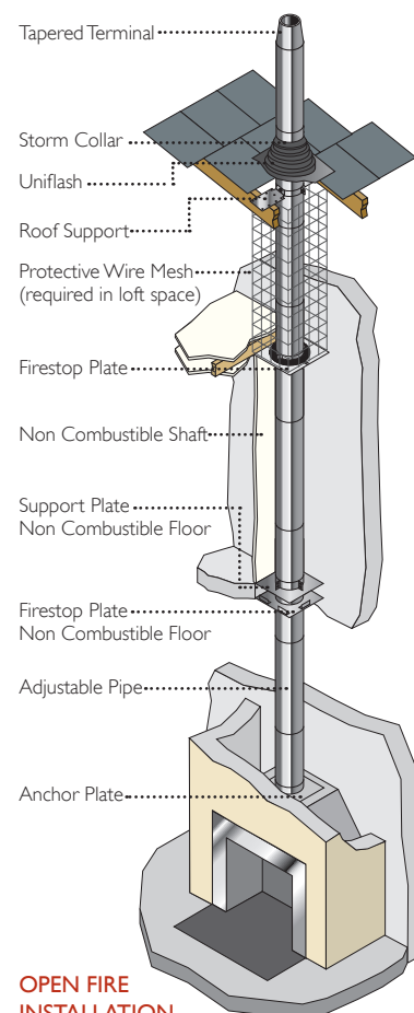
TYPICAL INSTALLATION USING ICS PLUS
