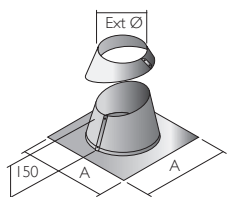
Angled Flashing Kit 5° - 45°
