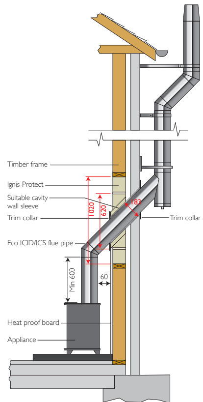
IGNIS-PROTECT ICS ON TRADITIONAL TIMBER FRAME WALL
