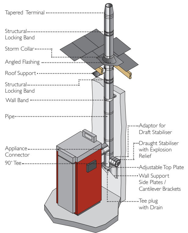
TYPICAL BIOMASS INSTALLATION FROM REAR OUTLET USING ICS SYSTEM CHIMNEY WITH 90° TEE SOLUTION
