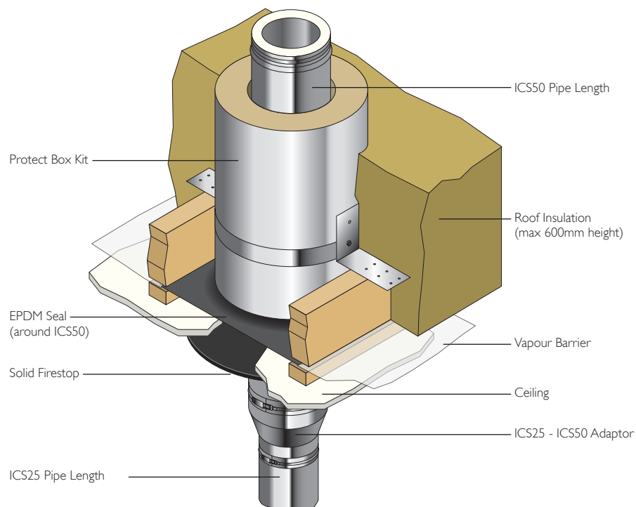
PROTECT BOX IN SITU
