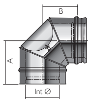
Inspection Bend
