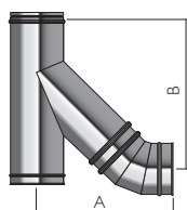
Offsets for 135° Tee & 45° Bend
